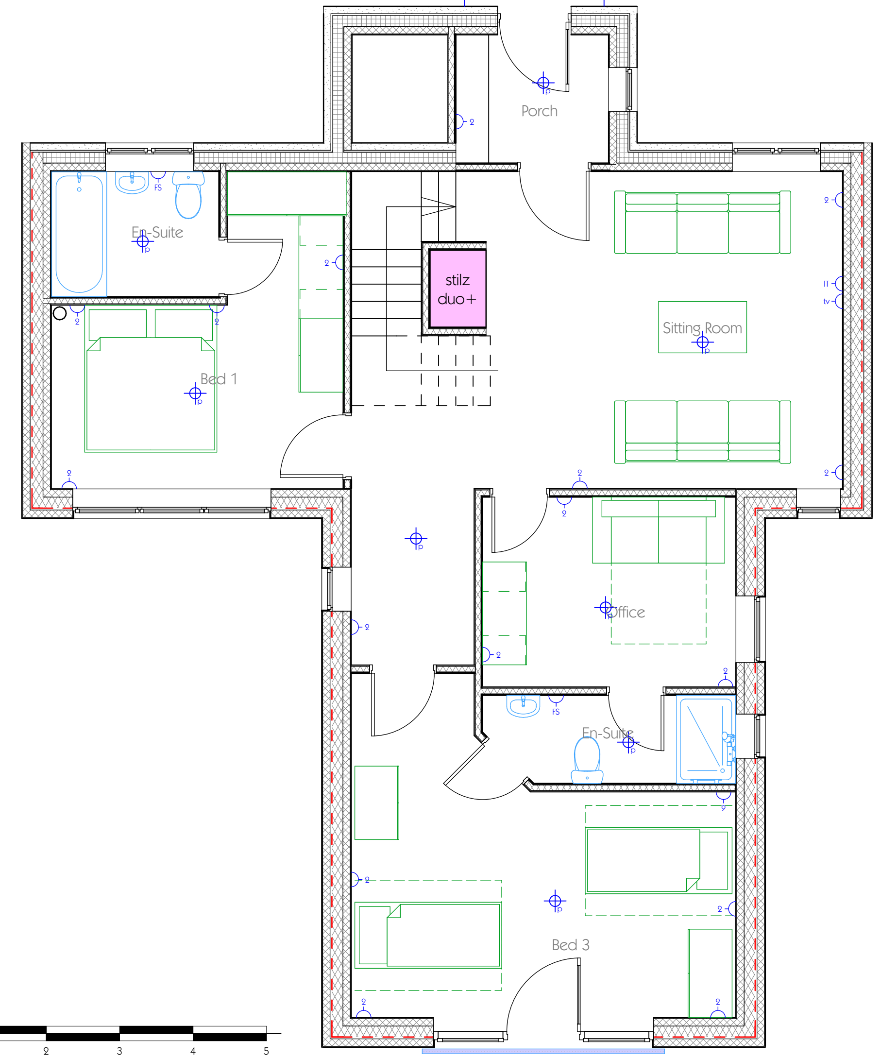
First Floor - Proposed layout
