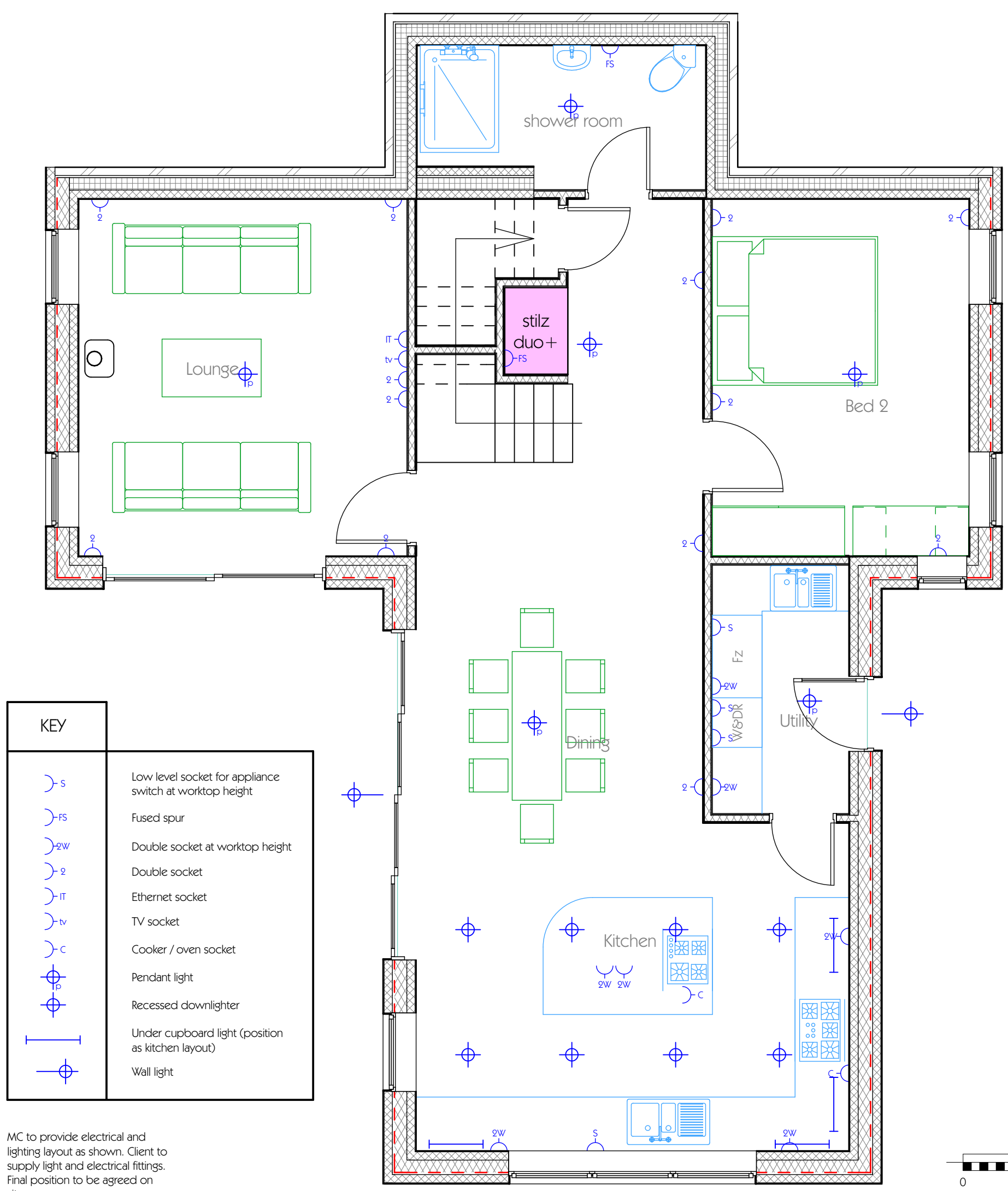
Ground Floor - Proposed layout
